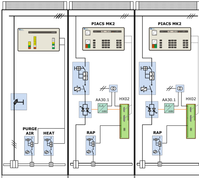
EXISTING PANEL WITH PIACS MK2
