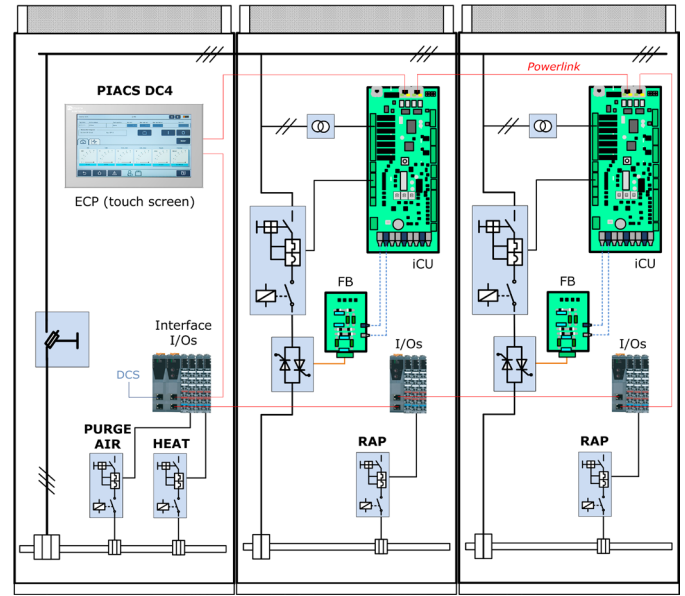
PIACS DC4 BUILT-IN EXISTING PANEL
