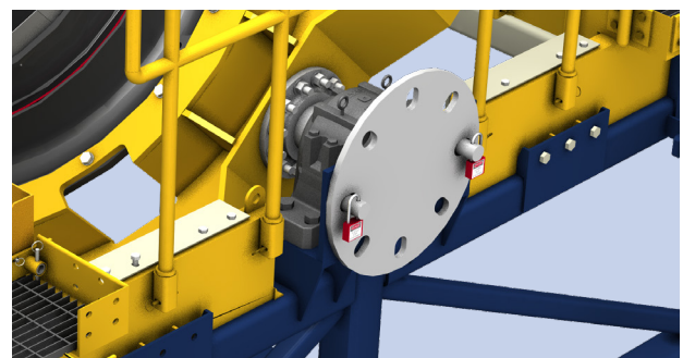
Gearbox driven rotating mechanism for full 360° rotation
